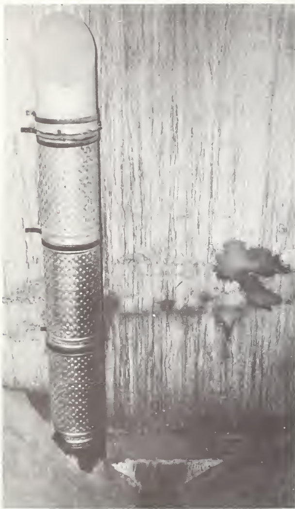
FIGURE 3.—Vertical aeration duct.
